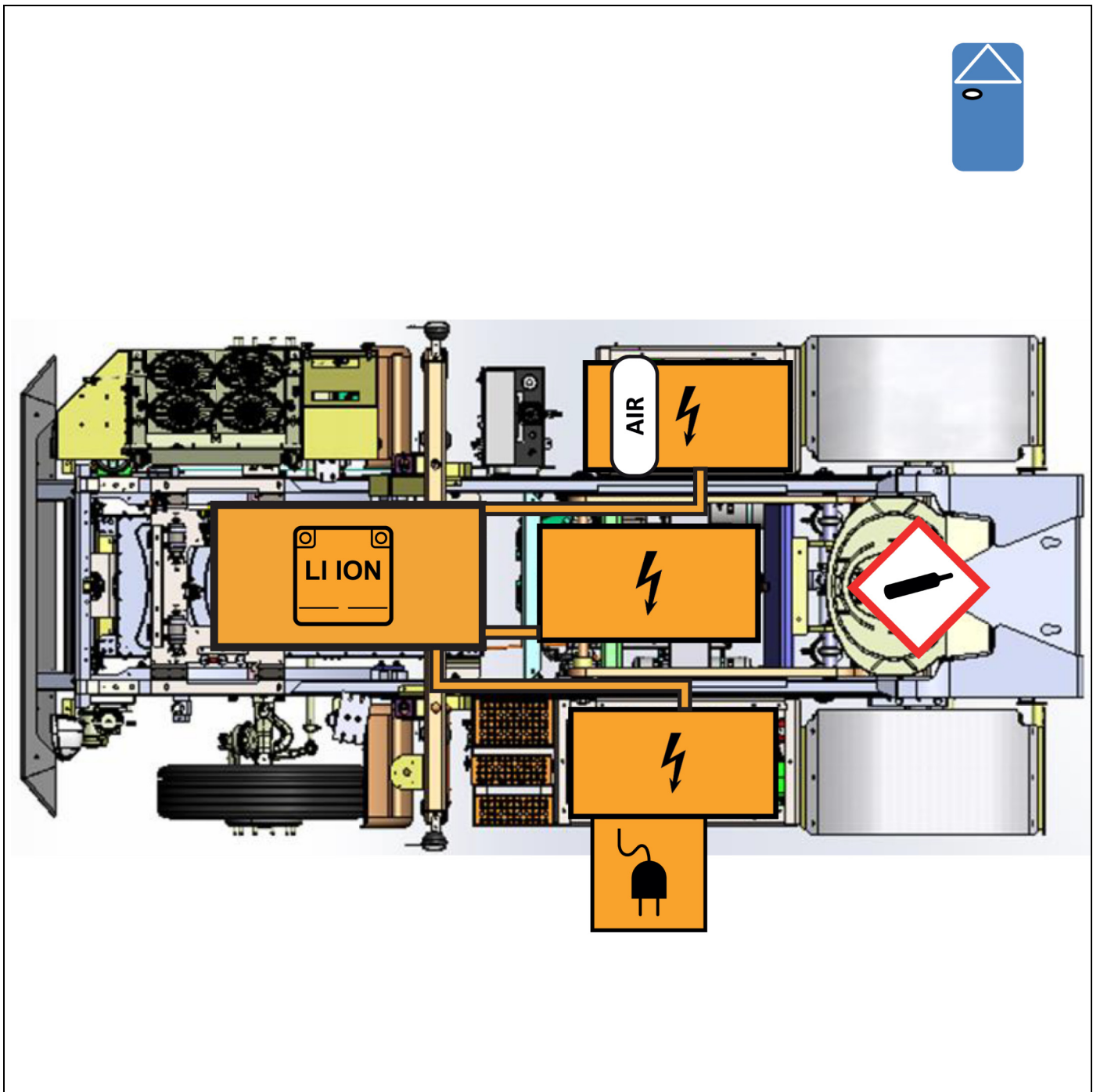
Figure 1-1: Top View
